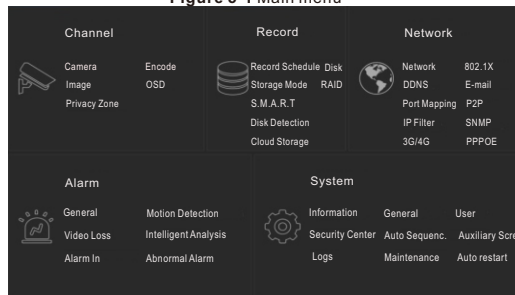
Figure 5-1 Main menu
